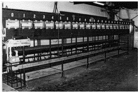
The "Tunnel Furnace" Test Apparatus used in the classification of materials as to their Surface Burning Characteristics.
