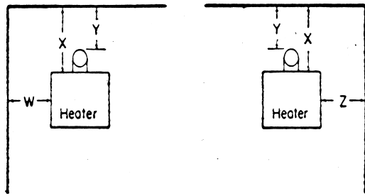
Figure 3 — Typical Room Heater Installation
